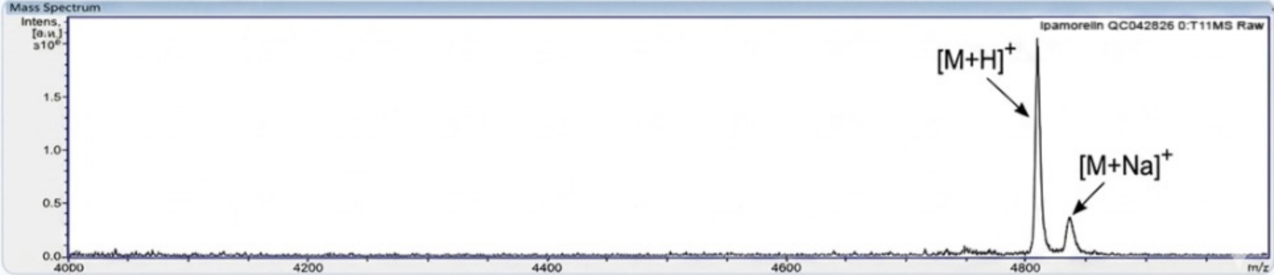
Mass Spectrum (MALDI-MS)
